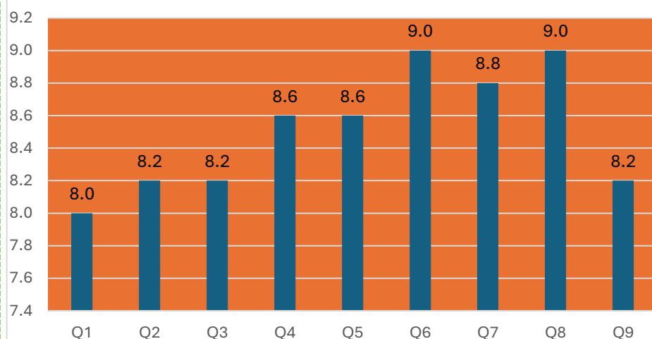
Solid Geometry
