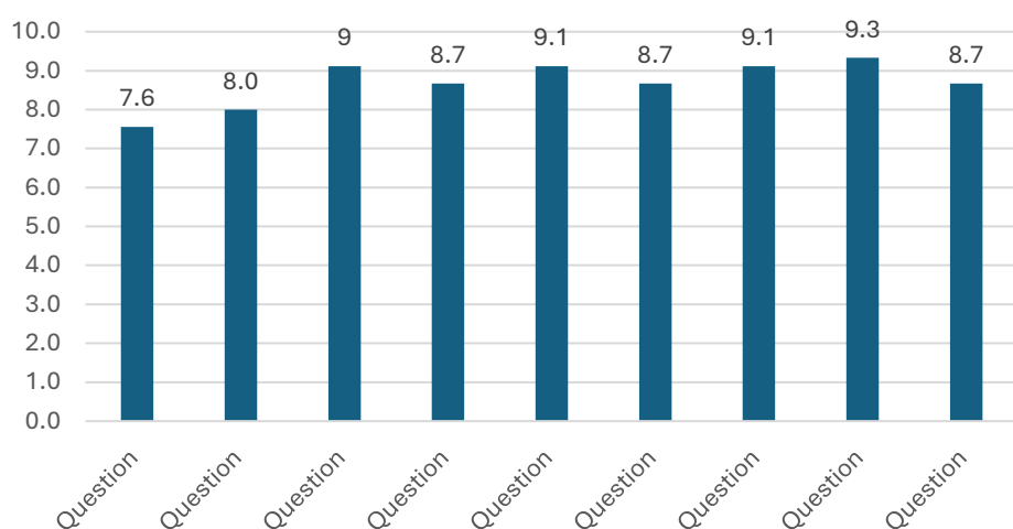
Laplace Transforms
